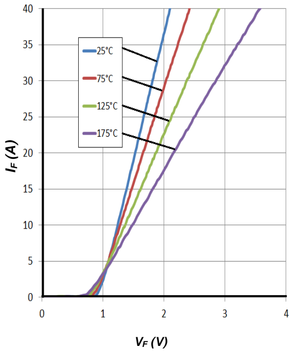
Figure 1. Forward Characteristics
