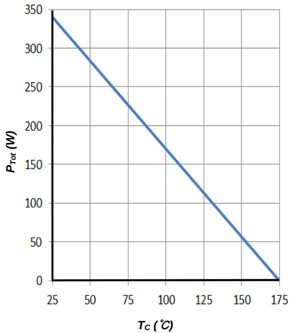
Figure 3. Power Derating
