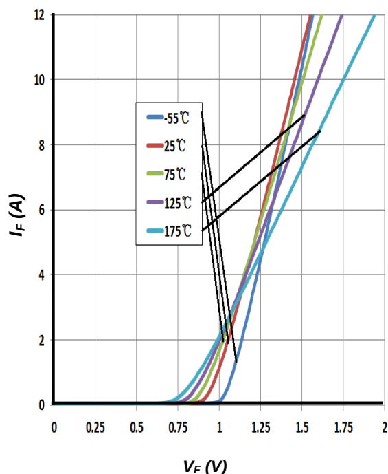
Figure 1. Forward Characteristics
