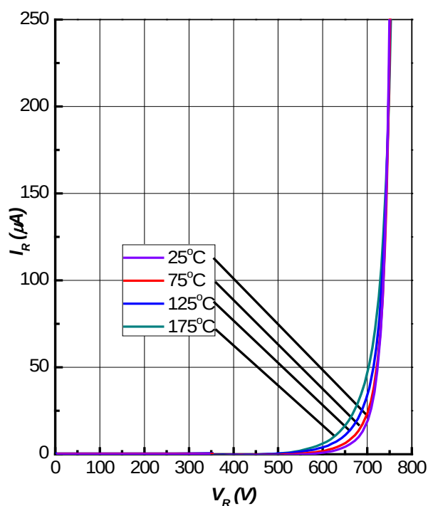
Figure 2. Reverse Characteristics
