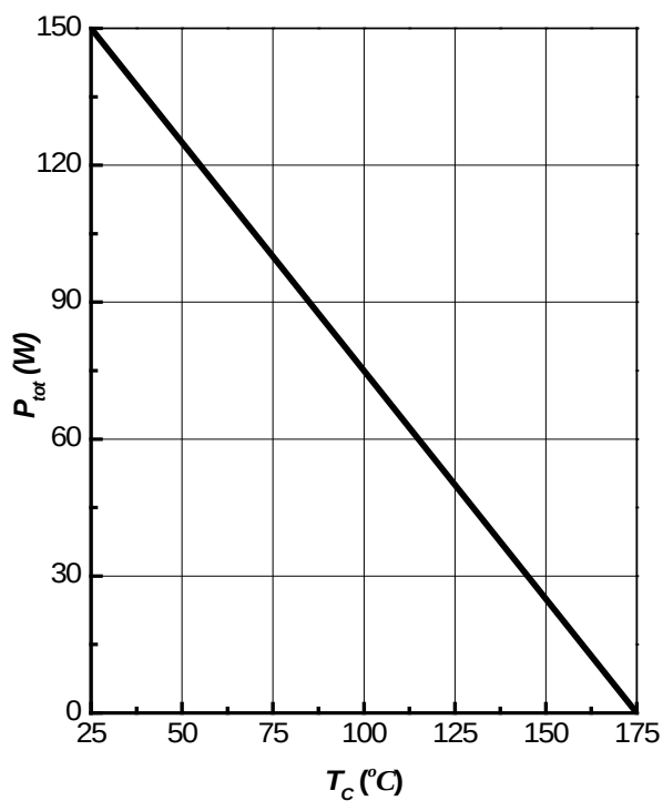
Figure 3. Power Derating
