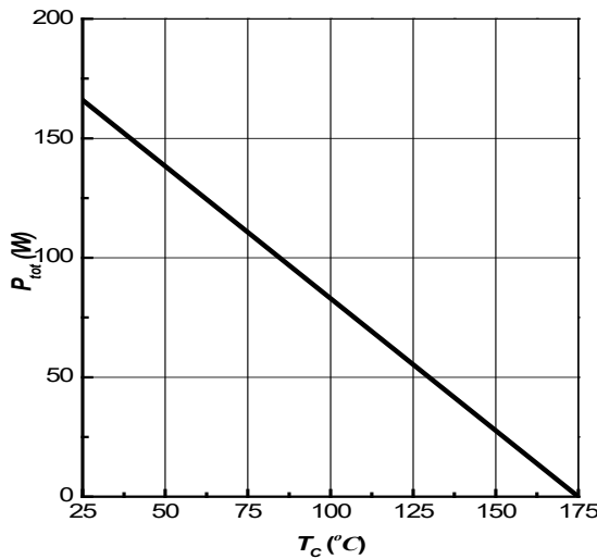
Figure 3. Power Derating
