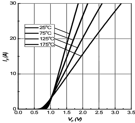
Figure 1. Forward Characteristics
