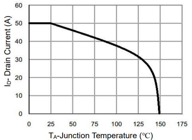
Figure 10 Current De-rating
