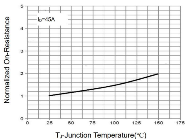
Figure 4 Rdson-Junction Temperature
