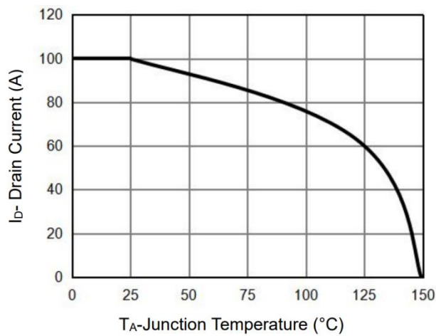
Figure 10 Current De-rating
