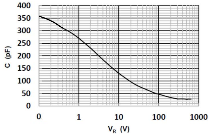
Figure 4. Typical capacitance as function of reverse voltage, C=f(V_R) ; T_j=25^\circ\text{C}
