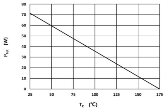
Figure 6. Power dissipation as function of case temperature
