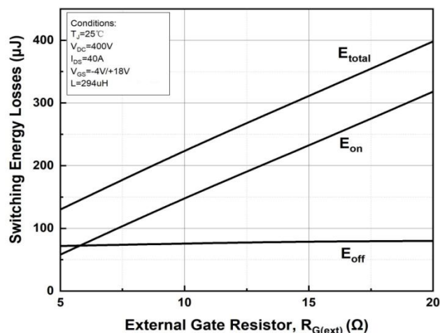
Figure 20. Clamped Inductive Switching Energy vs. R_{G(\text{ext})}
