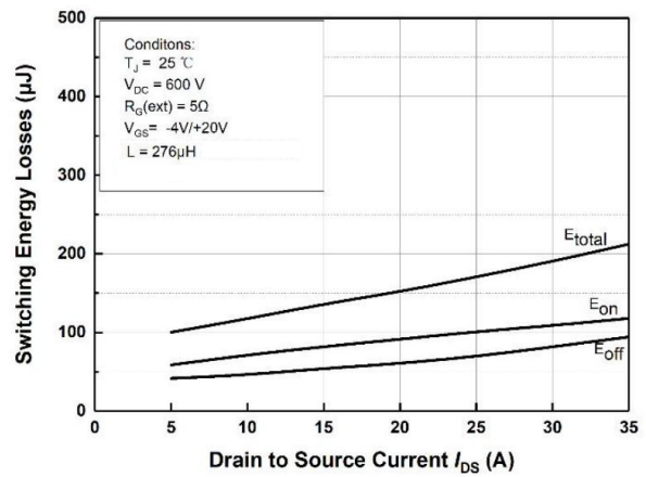
Figure 20. Clamped Inductive Switching Energy vs. Drain Current( V_{DD} = 600\text{V} )
