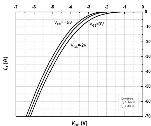
Figure 8. Body Diode Characteristics at T_j=175^{\circ}\text{C}
