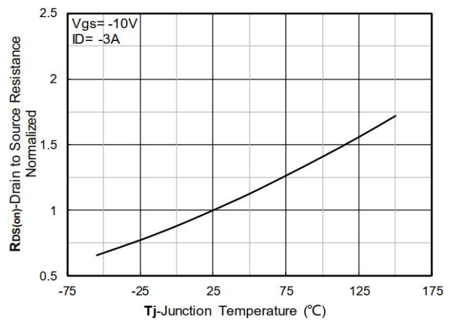
Figure 6. Normalized On-Resistance
