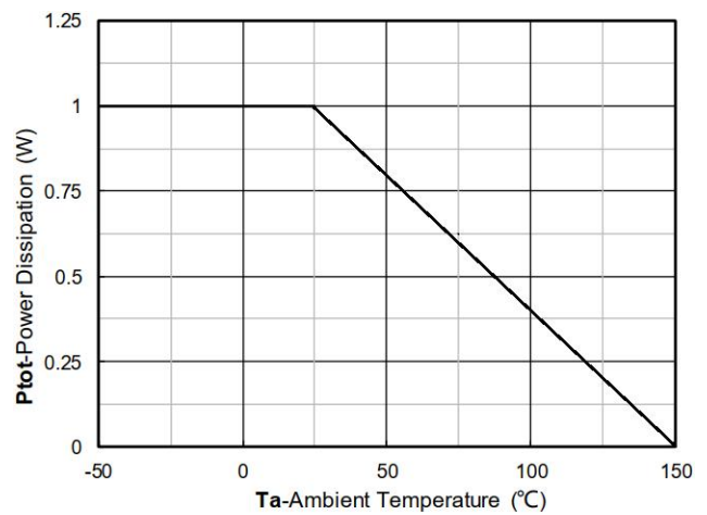
Figure 12. Power dissipation
