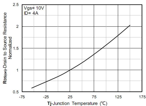
Figure 6. Normalized On-Resistance
