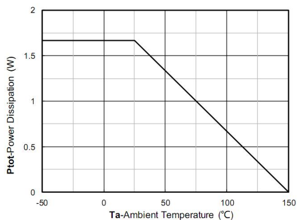
Figure 12. Power dissipation
