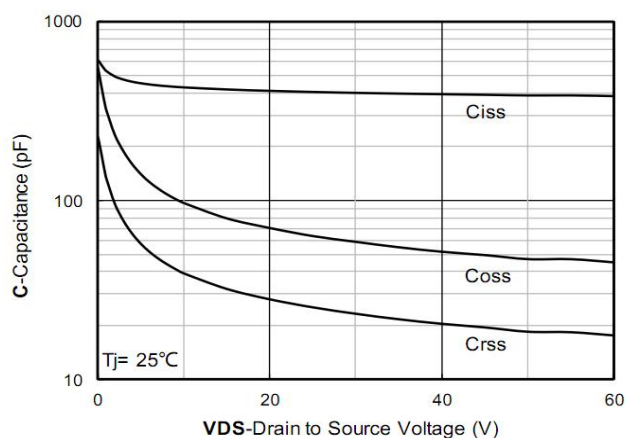
Figure 3. Capacitance Characteristics
