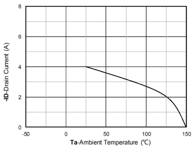
Current dissipation
