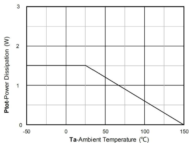
Power dissipation
