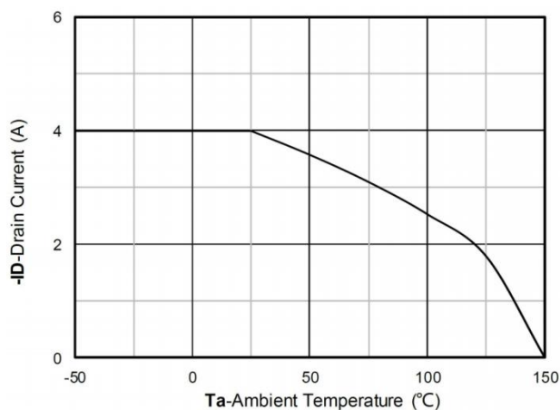
Current dissipation
