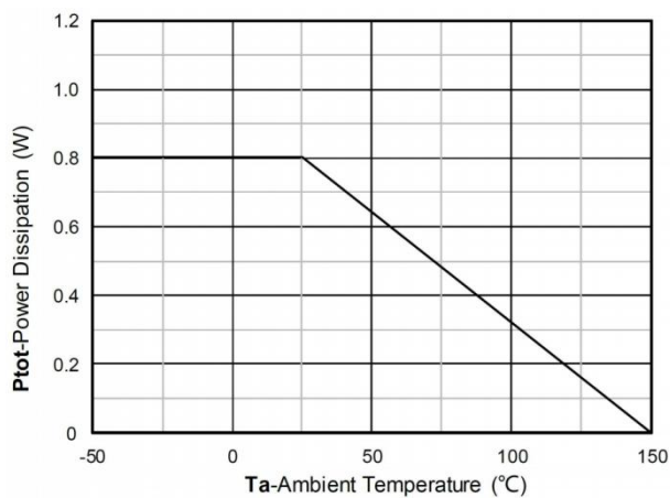
Power dissipation
