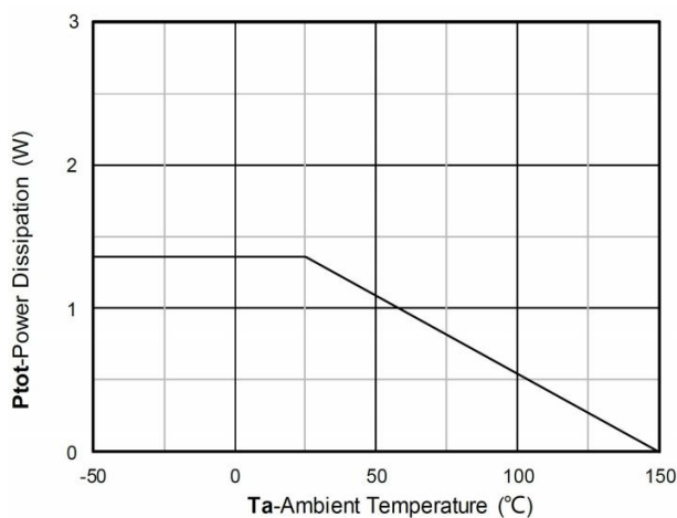
Power dissipation
