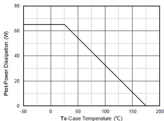
Figure 12. Power dissipation
