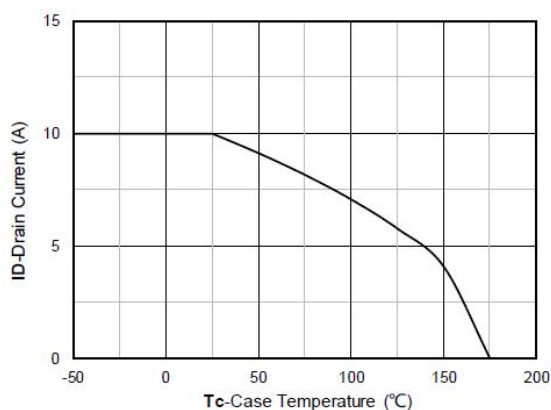
Figure 11. Current dissipation
