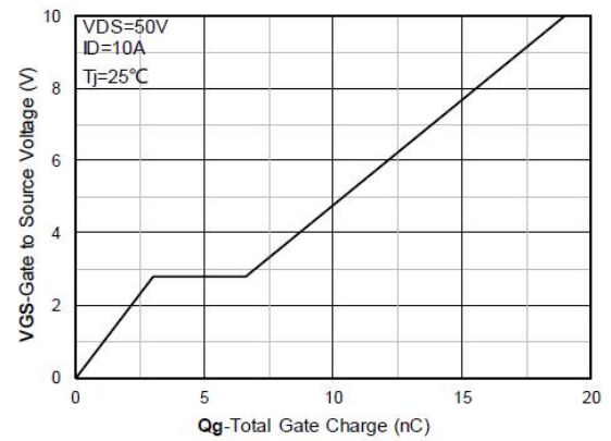
Figure 4. Gate Charge
