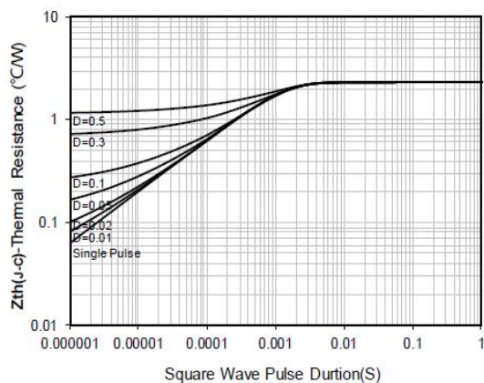
Figure 13. Maximum Transient Thermal Impedance
