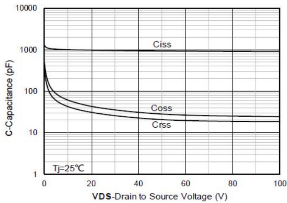
Figure 3. Capacitance Characteristics
