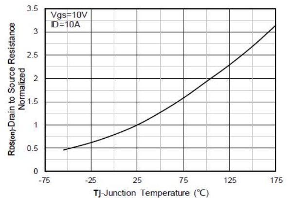
Figure 6. Normalized On-Resistance
