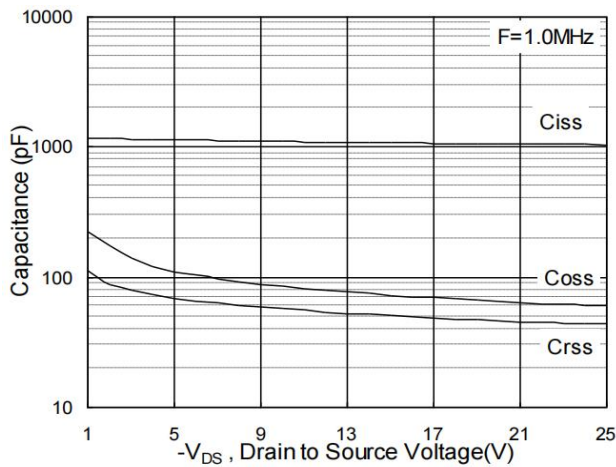
Fig.7 Capacitance
