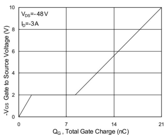
Fig.4 Gate-Charge Characteristics
