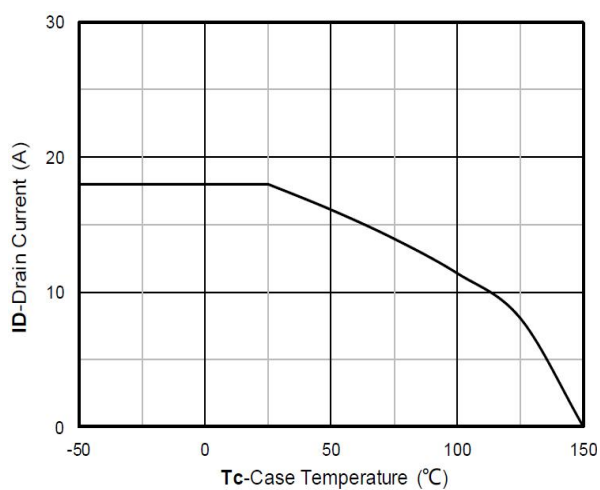
Figure 11. Current dissipation
