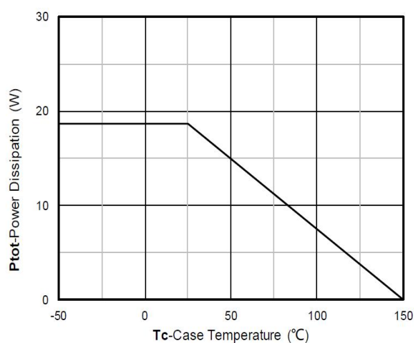
Figure 12. Power dissipation
