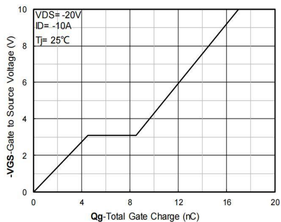
Figure 4. Gate Charge
