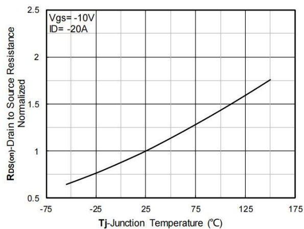
Figure 6. Normalized On-Resistance
