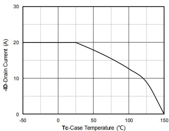
Figure 11. Current dissipation
