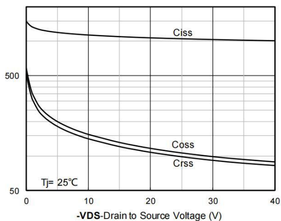
Figure 3. Capacitance Characteristics
