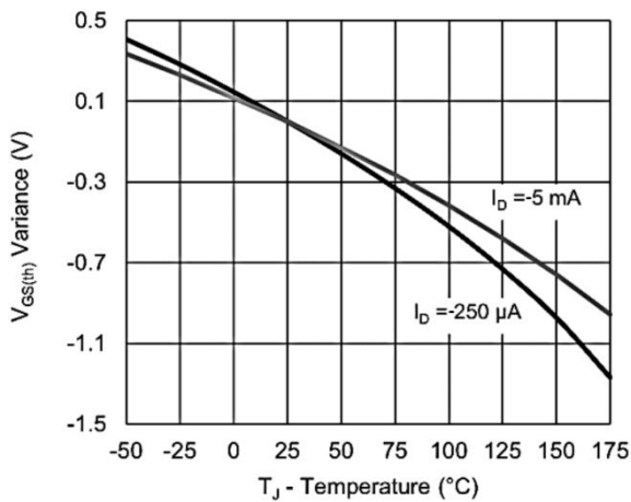
Fig9: Threshold Voltage
