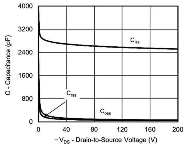
Fig4: Capacitance
