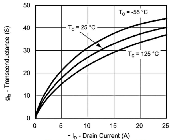
Fig2: Transfer Characteristics
