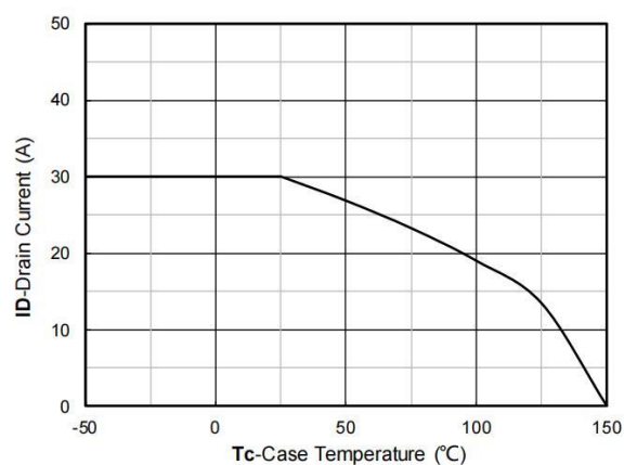
Figure 11. Current dissipation
