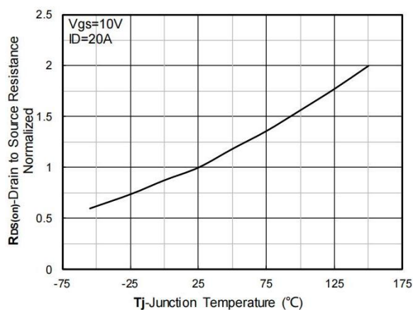
Figure 6. Normalized On-Resistance
