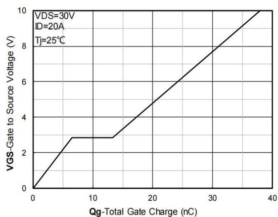
Figure 4. Gate Charge
