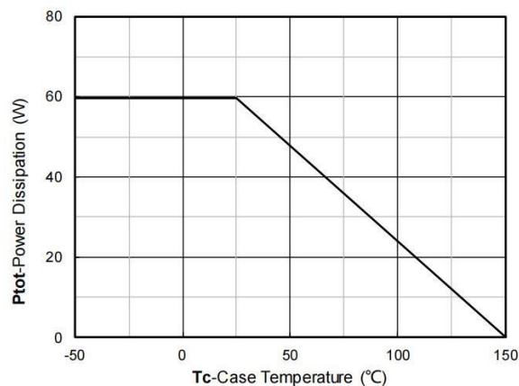
Figure 12. Power dissipation
