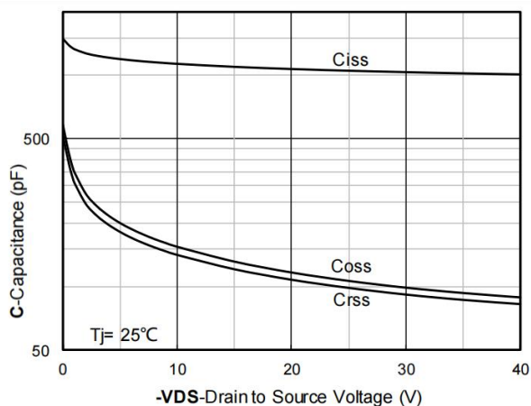
Figure 3. Capacitance Characteristics
