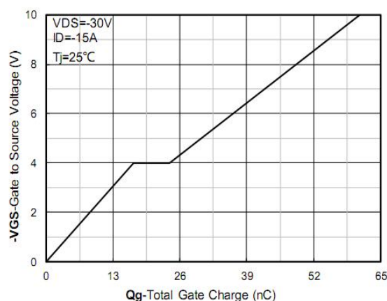
Figure 4. Gate Charge
