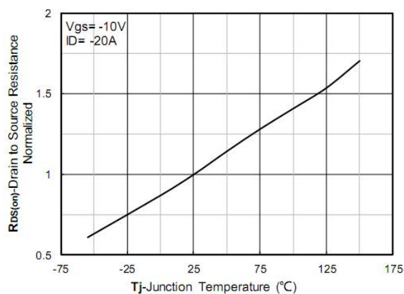
Figure 6. Normalized On-Resistance
