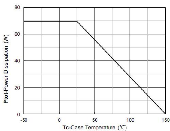
Figure 12. Power dissipation
