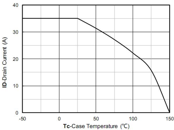
Figure 11. Current dissipation
