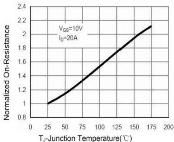
Rdson-Junction Temperature
