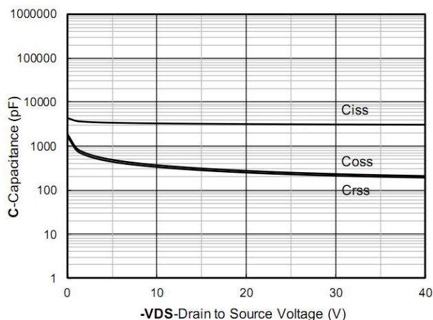
Figure 3. Capacitance Characteristics
