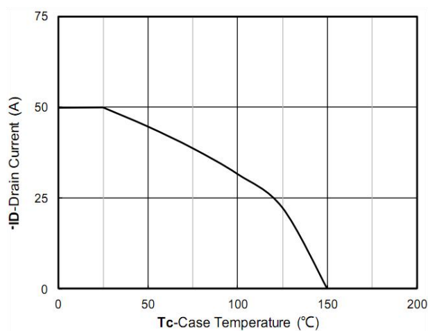
Figure 11. Current dissipation
