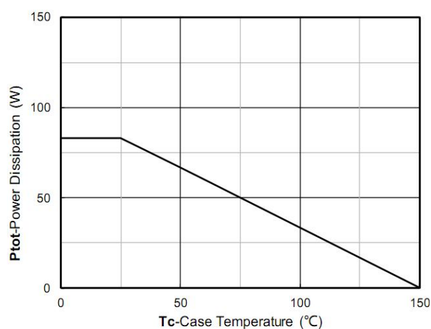
Figure 12. Power dissipation
