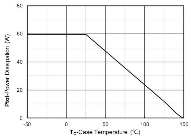
Figure 12. Power dissipation
