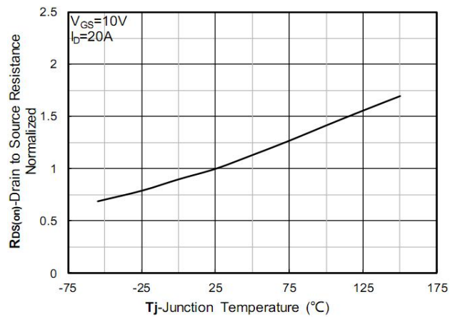
Figure 6. Normalized On-Resistance
