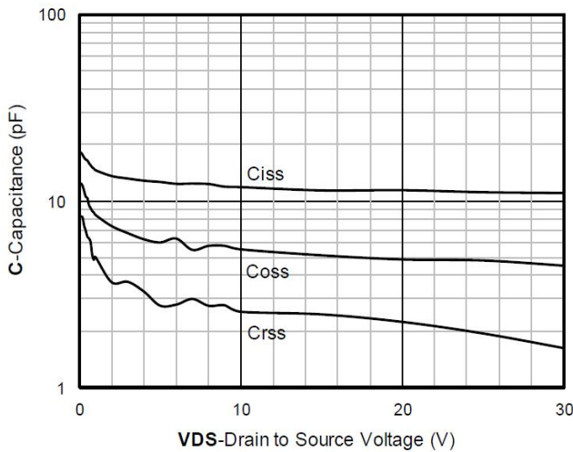
Figure 3. Capacitance Characteristics
