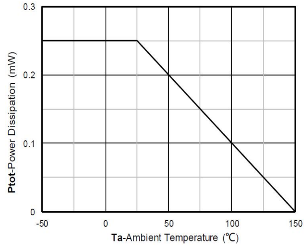
Figure 12. Power dissipation
