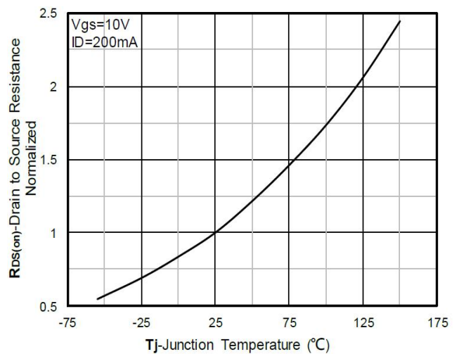
Figure 6. Normalized On-Resistance
