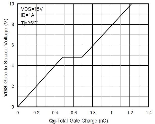
Figure 4. Gate Charge
