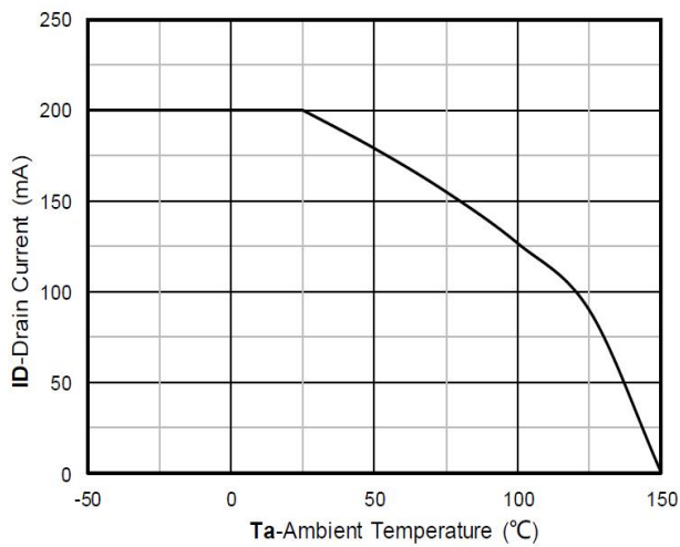
Figure 11. Current dissipation
