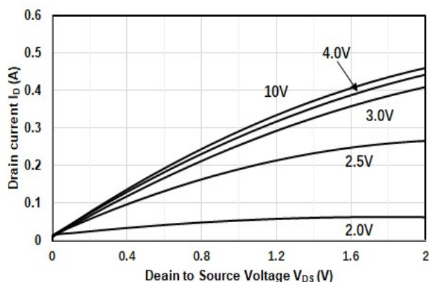
Figure1. Output Characteristics
