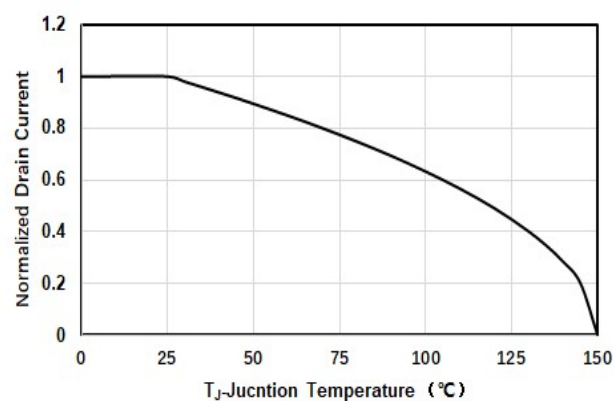
Figure8. Drain-Source Current
