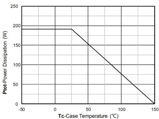
Power dissipation
