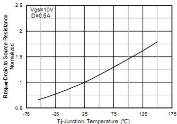
Figure 6. Normalized On-Resistance
