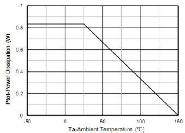
Figure 12. Power dissipation
