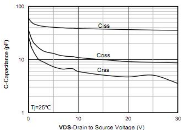
Figure 3. Capacitance Characteristics
