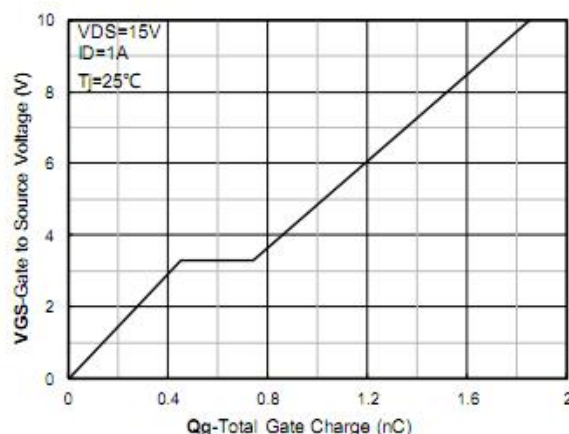
Figure 4. Gate Charge
