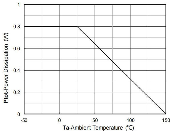
Figure 12. Power dissipation
