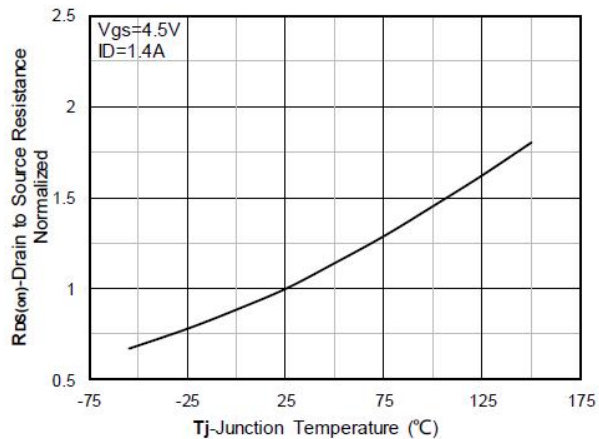
Figure 6. Normalized On-Resistance
