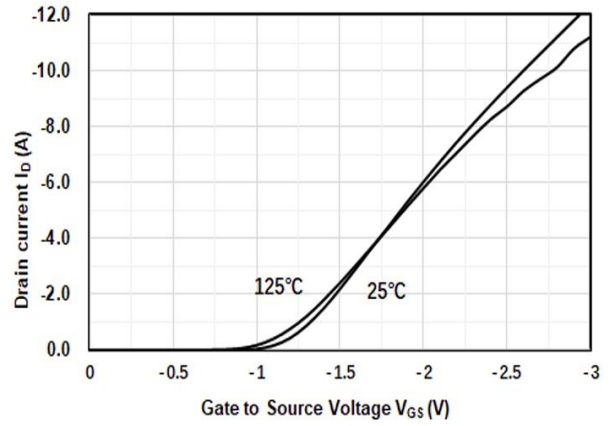
Figure2. Transfer Characteristics
