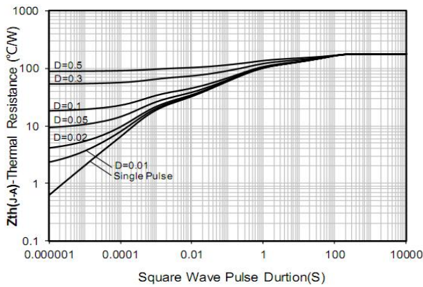
Figure9. Maximum Transient Thermal Impedance
