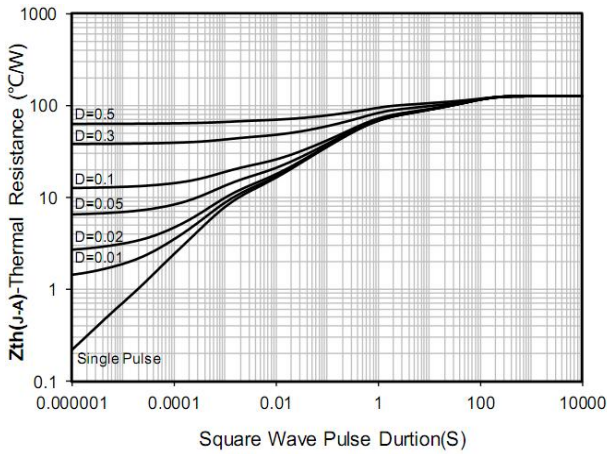
Figure9. Maximum Transient Thermal Impedance
