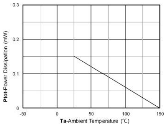
Power dissipation
