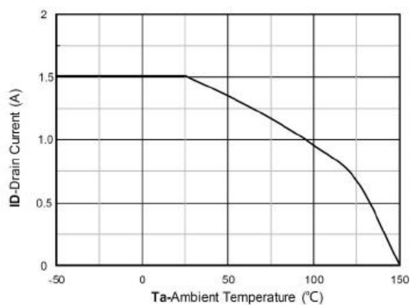
Current dissipation
