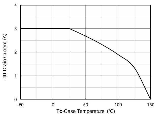
Figure 11. Current dissipation
