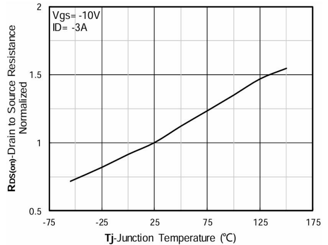
Figure 6. Normalized On-Resistance
