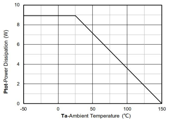
Figure 12. Power dissipation
