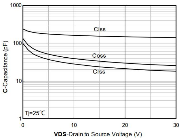
Figure 3. Capacitance Characteristics
