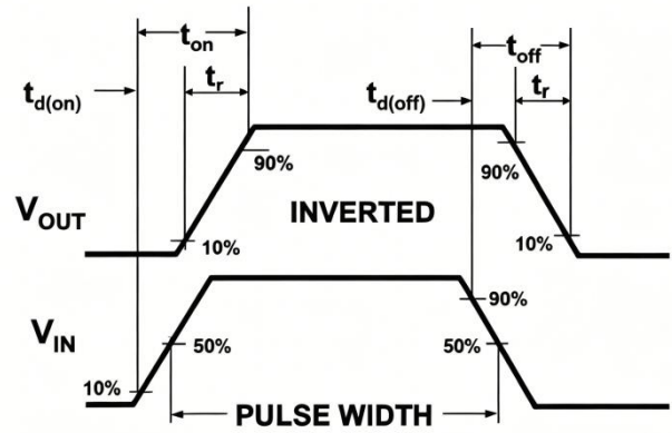
Figure8. Switching wave
