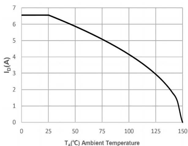
Maximum Continuous Drain Current vs. Ambient Temperature
