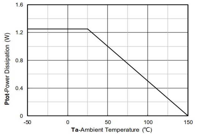
Figure 12. Power dissipation
