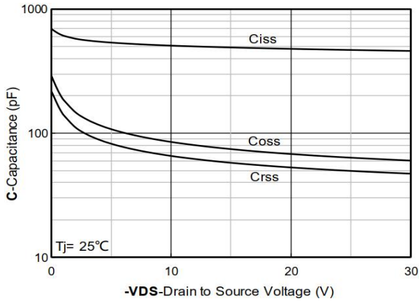
Figure 3. Capacitance Characteristics
