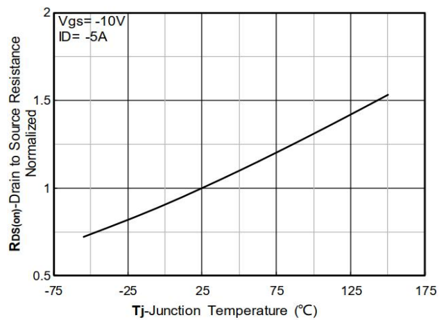
Figure 6. Normalized On-Resistance
