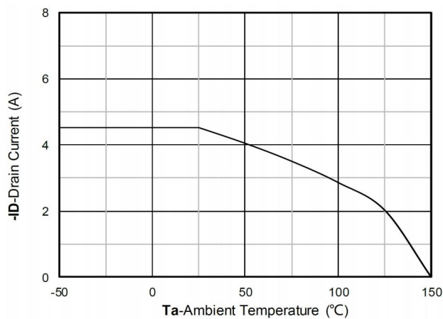
Current dissipation
