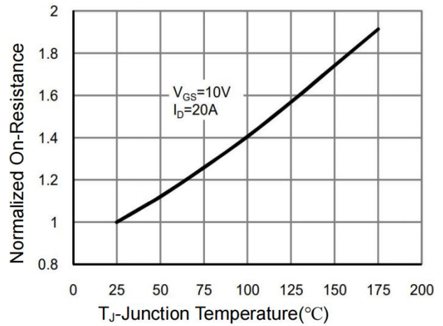
Figure 4 Rdson-Junction Temperature
