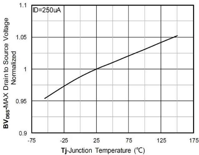
Normalized breakdown voltage
