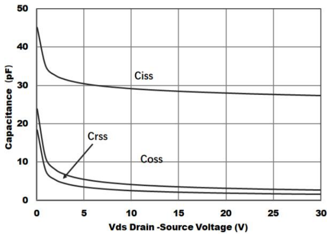
Figure3. Capacitance Characteristics
