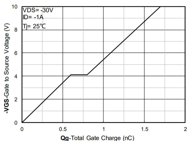
Figure 4. Gate Charge
