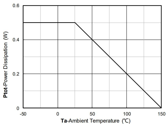
Figure 12. Power dissipation
