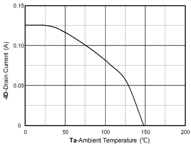
Current dissipation
