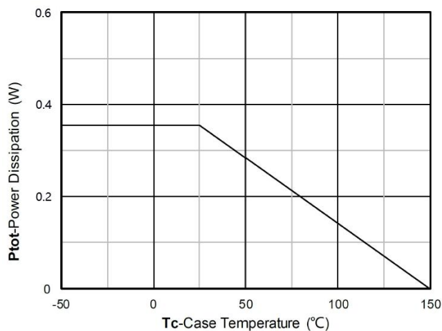
Power dissipation
